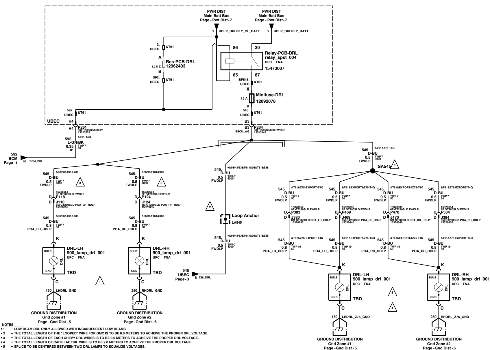
Lights-Exterior: Headlamps/Parklamps Headlamps LE01 Panel 6 of 7
